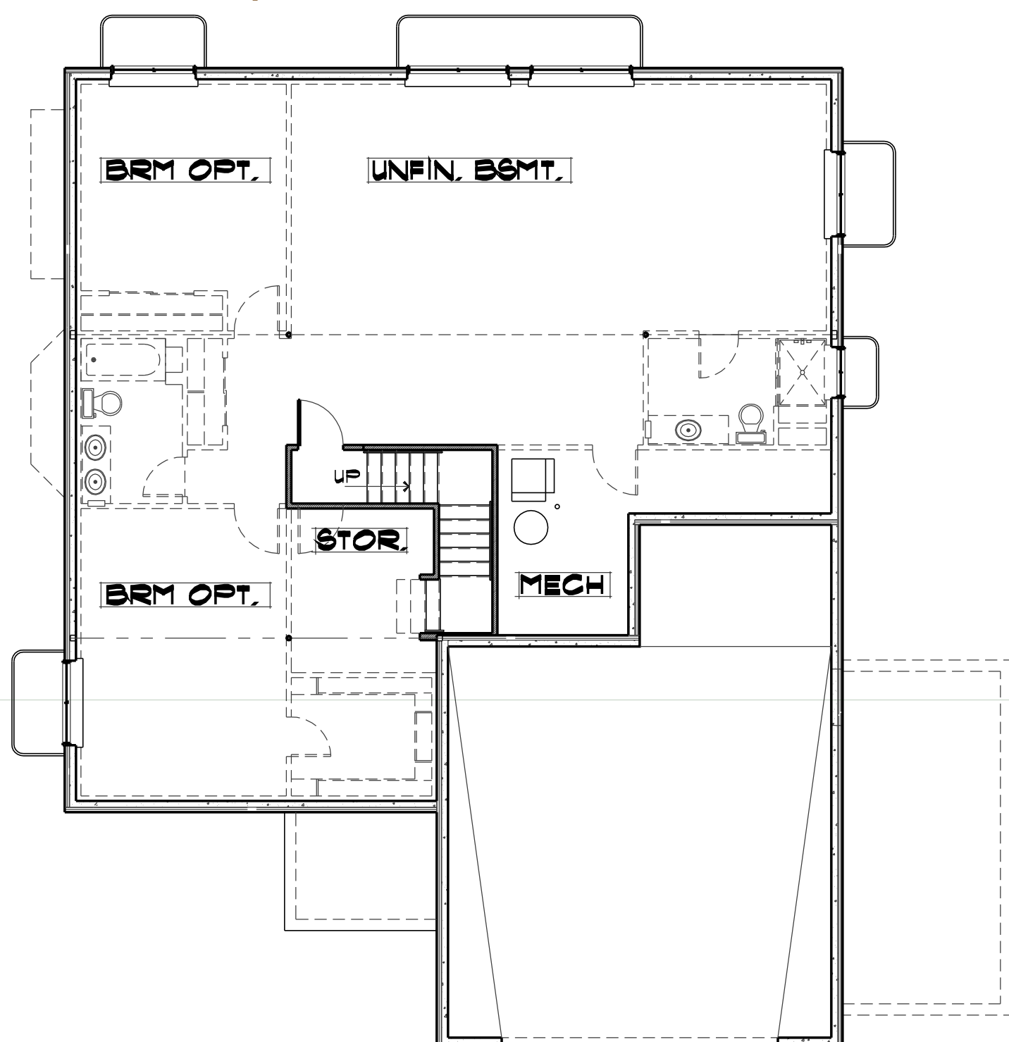
156 - Lower Level Floor Plan
