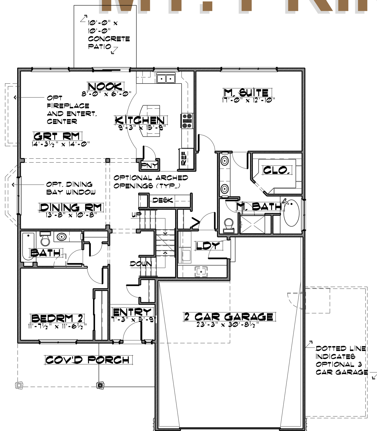
156 - Main Level Floor Plan
